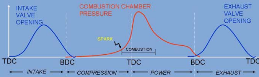
4T Timing Diagram
